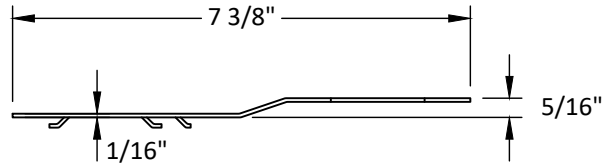
3 ANCHOR STRAP
