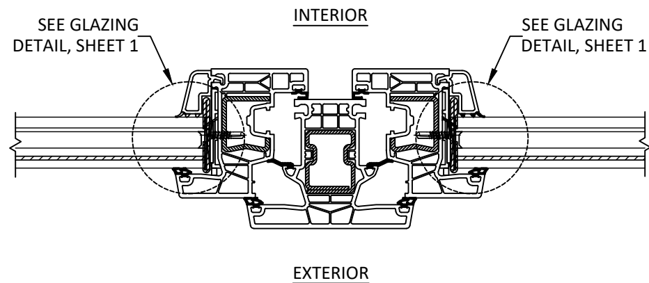
D 3 HORIZONTAL SECTION VERTICAL INTEGRAL POST
