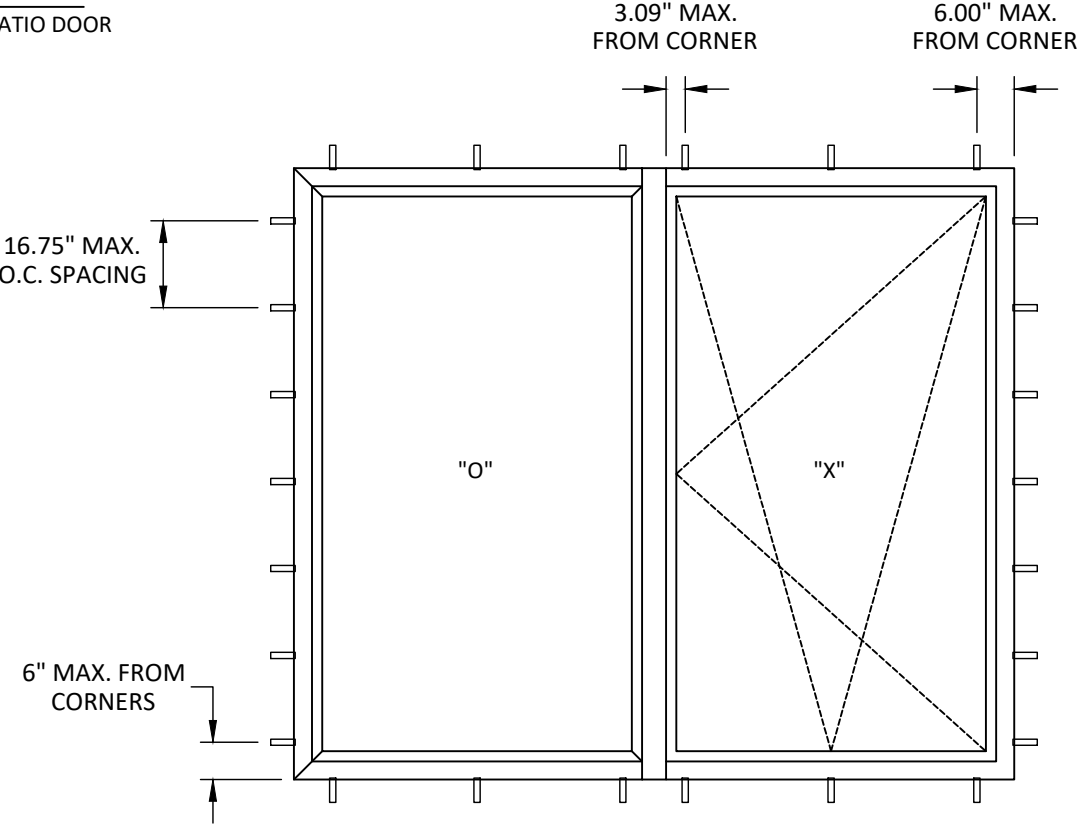
ANCHOR LAYOUT ANCHOR STRAP
