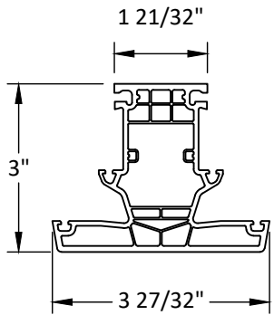
5 MULLION
