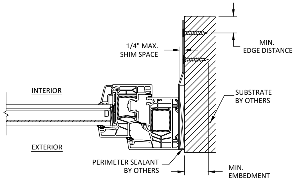
B 4 ANCHOR DETAIL STRAP (JAMB)
